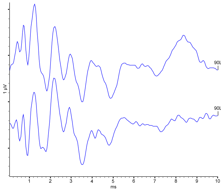
Chart 1 -- Waveforms
